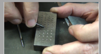
SHARPENING A BEADING TOOL
